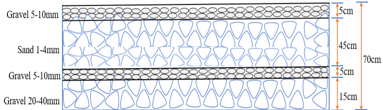
Figure 14: General view of media arrangement in HFCWs
