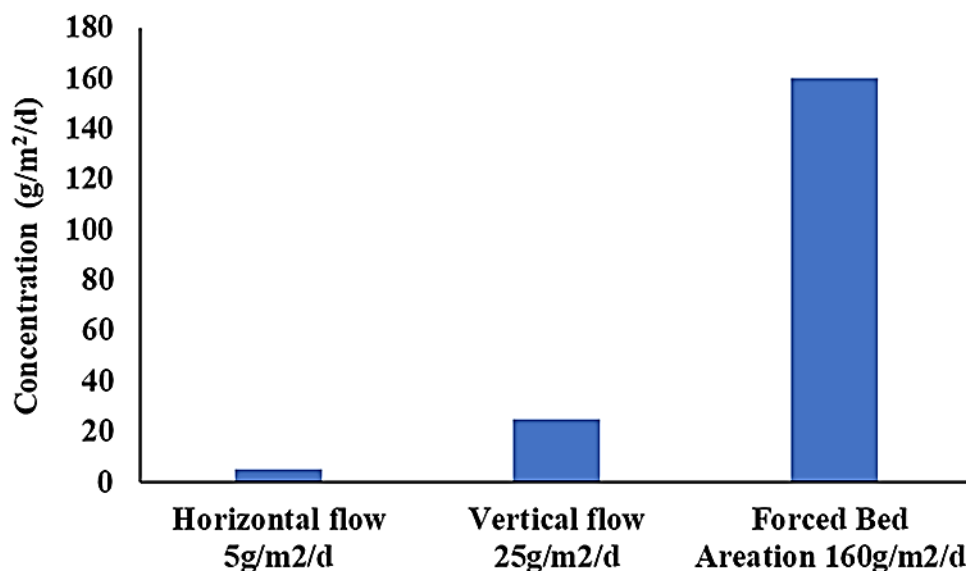
Figure 12: Comparison of oxygen transfer rates in CWs (Source: Personal communication Sh. Ganges Reddy, dated- August 22, 2023)
