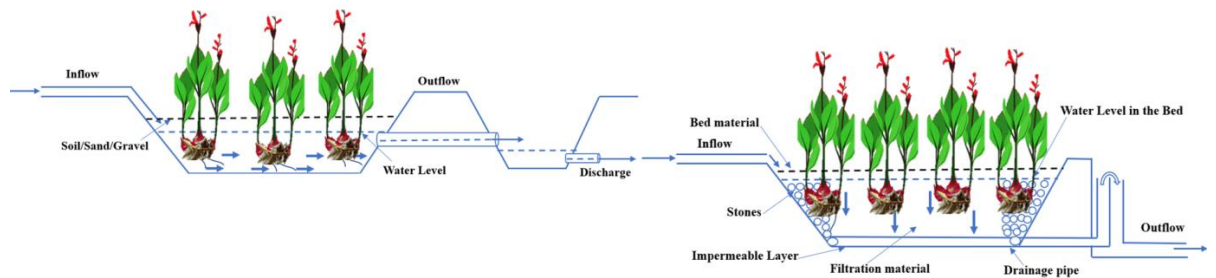
Figure 5: Basic design configuration of hybrid constructed wetlands
