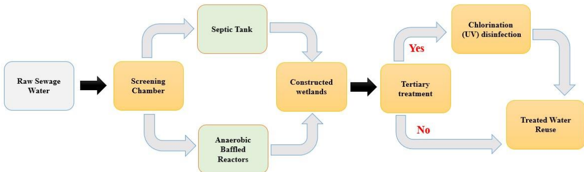
Figure 11: Integrated treatment set up with CWs
