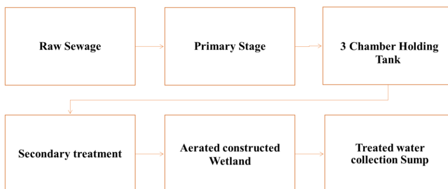
Figure: Process flow diagram
