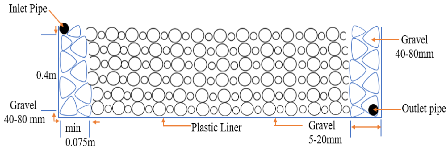
Figure 14: General view of media arrangement in HFCWs
