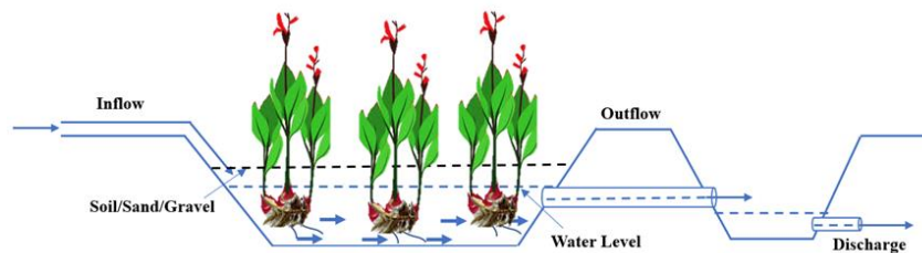
Figure 3: Basic design configuration of horizontal flow constructed wetlands
